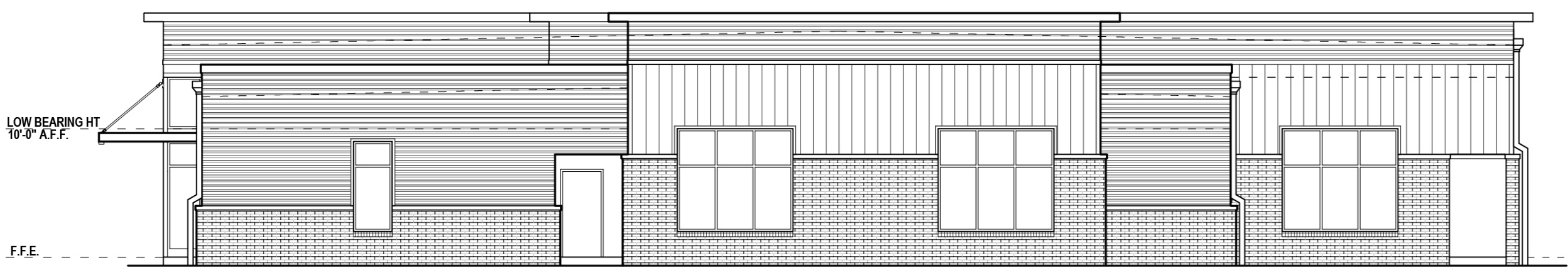
COMMON BUILDING RIGHT ELEVATION 1/8" = 1'-0"
