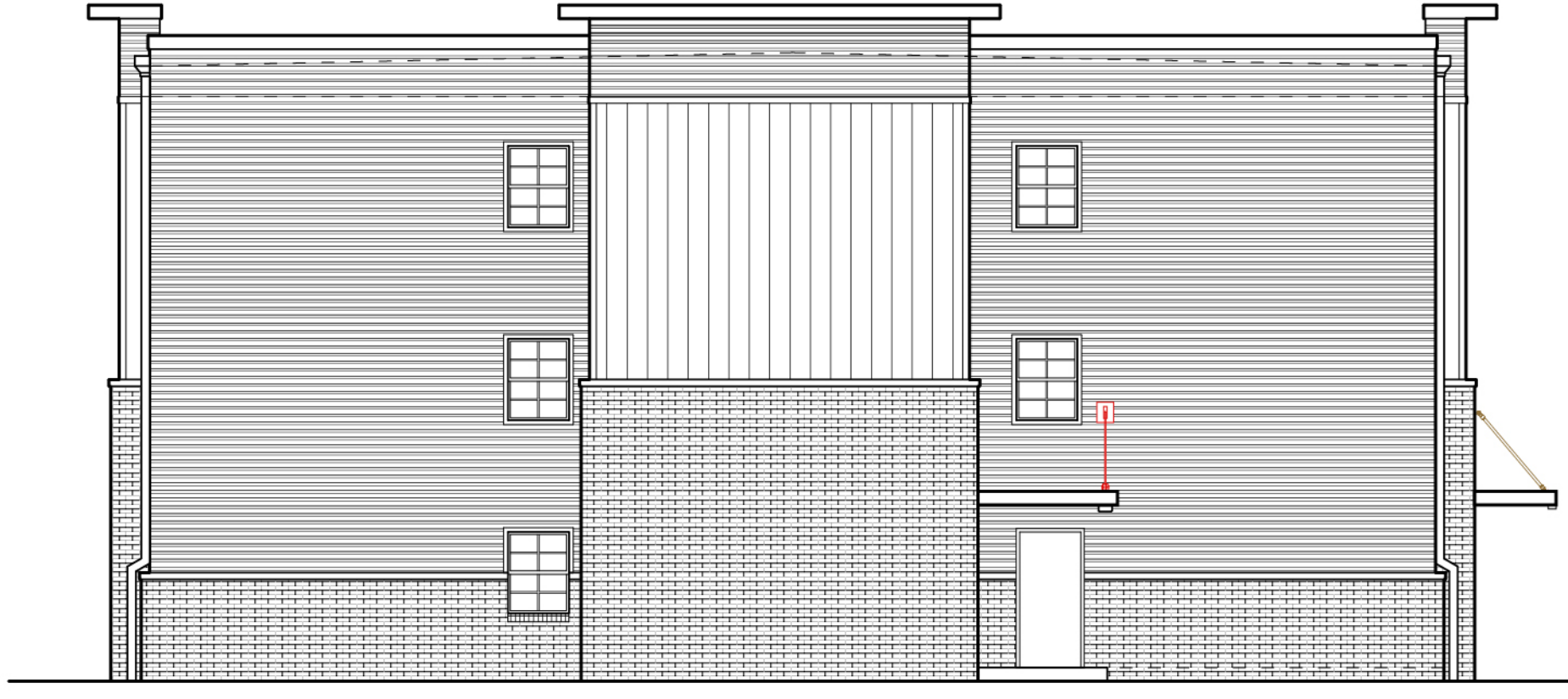
LIVING BUILDING LEFT ELEVATION 1/8" = 1'-0"
